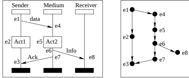
Fig. 2 An MSC Example and its underlying partial order
